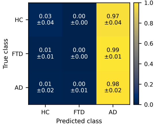
(a) GLM-5: mean \pm SD across five seeds
