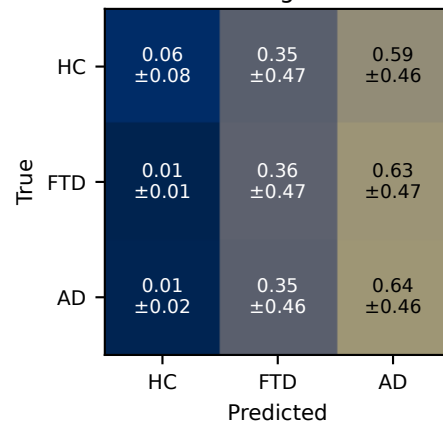
Qwen3-235B-A22B Thinking 2507
