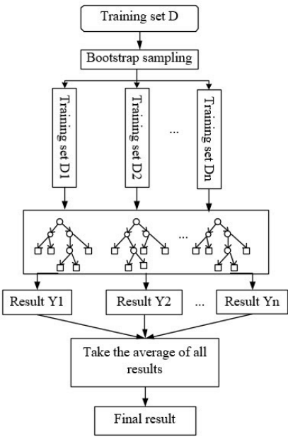
Gambar 2.2 Struktur Umum Random Forest Regression zhou2020pest
