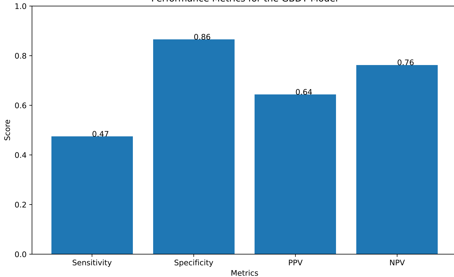
Performance Metrics for the GBDT Model
