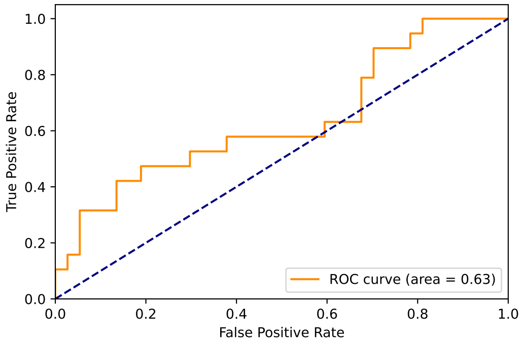
Receiver Operating Characteristic for Best Ablated Model
