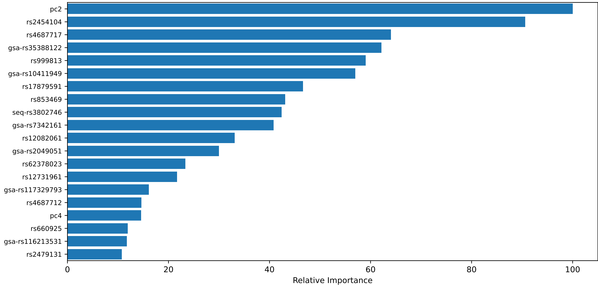
Top 20 Variable Importance
