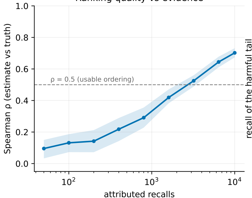
Ranking quality vs evidence
