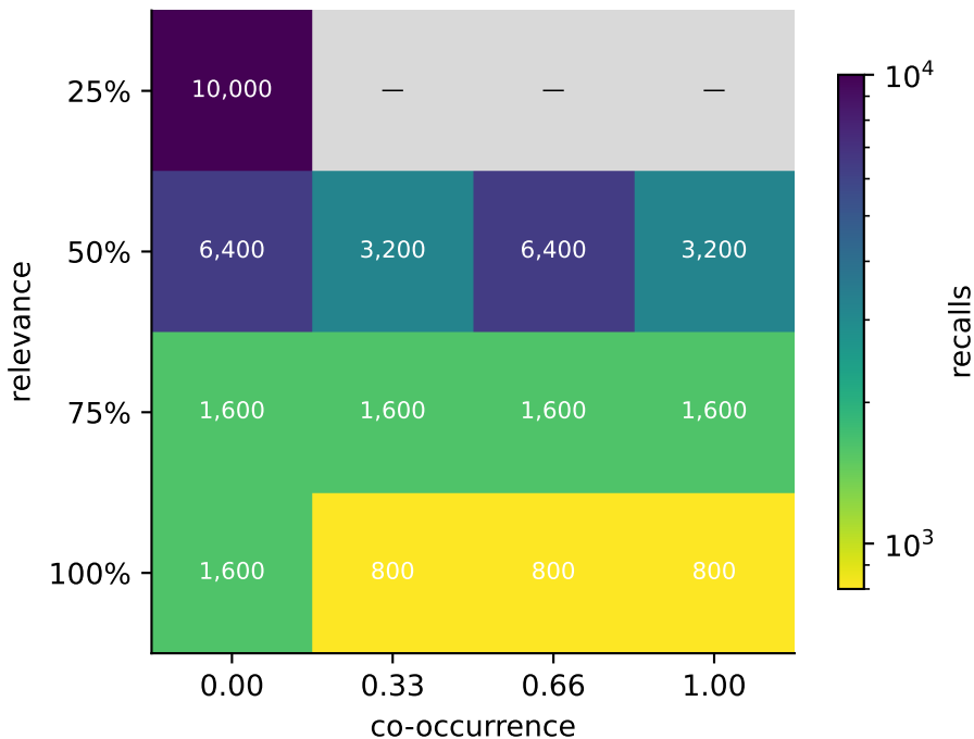
Recalls needed to reach \rho = 0.5 (grey = not reached within 10,000)
