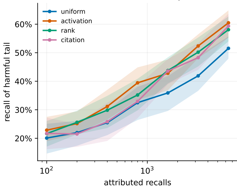
Quarantine accuracy
