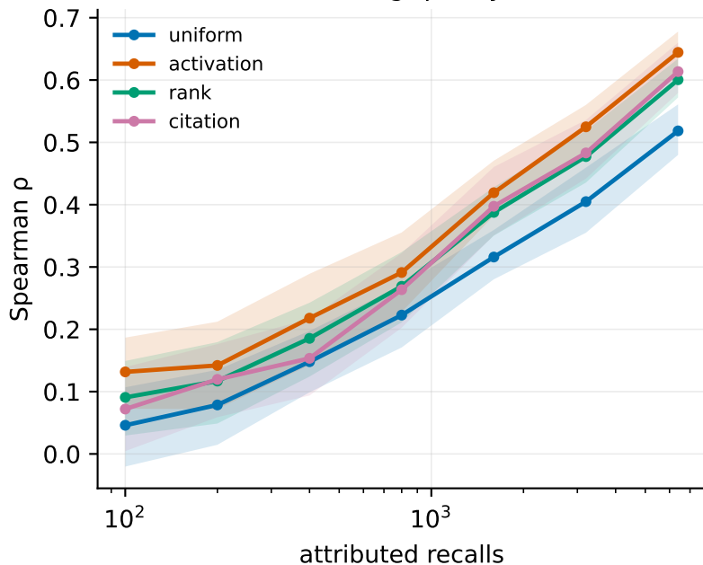
Ranking quality
