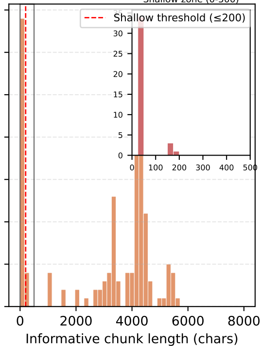
Pipeline B (Markdown) 38/150 shallow = 25.3% Shallow zone (0-500)
