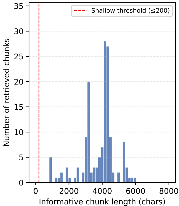
Pipeline A (Raw) 0/150 shallow = 0.0%
