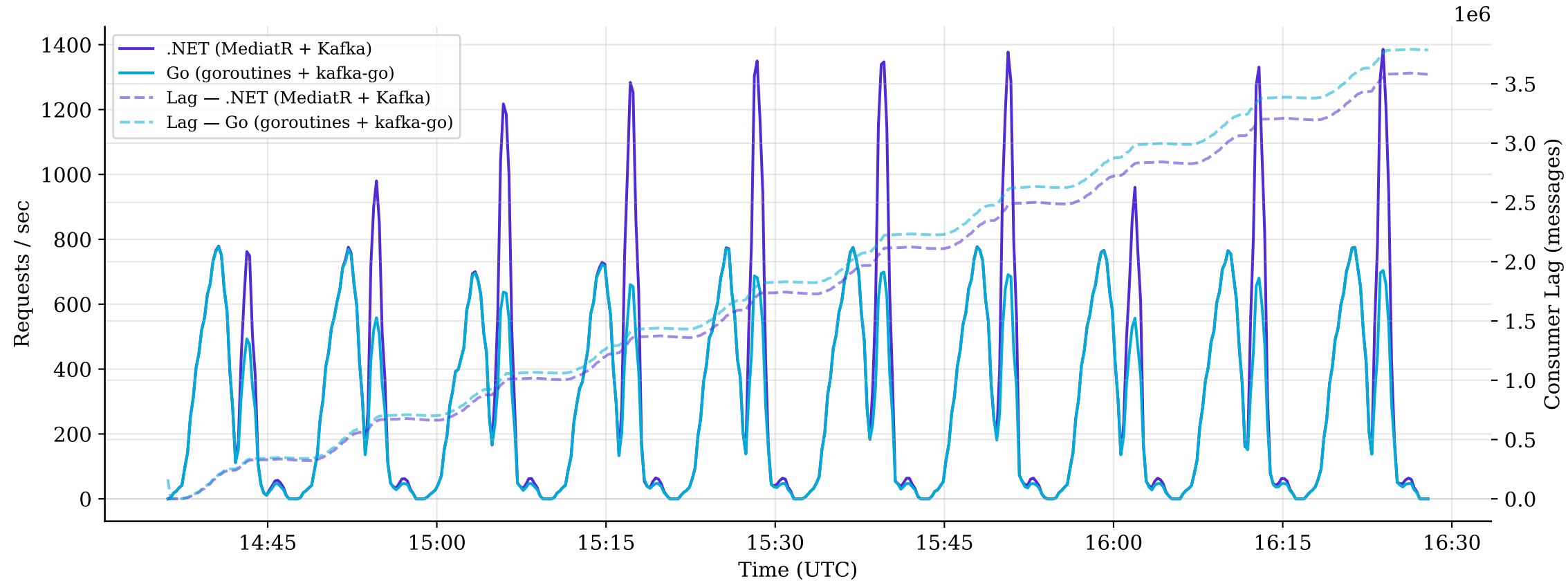
Throughput and Consumer Lag Over Time
