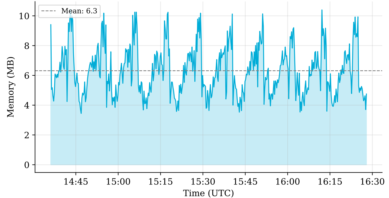
Heap — Go
