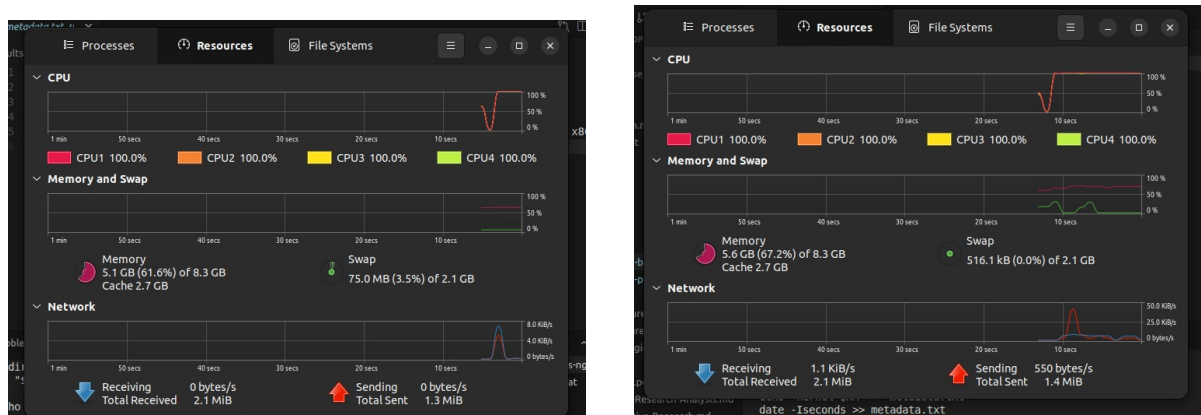
Figure 11. Left: representative benchmark / monitoring session on the baseline kernel during a stress-ng memory workload. Right: comparable session on the PressurePause kernel (same host class of workload; 120 s timeouts and tool output as in ./bench-run.sh ).
