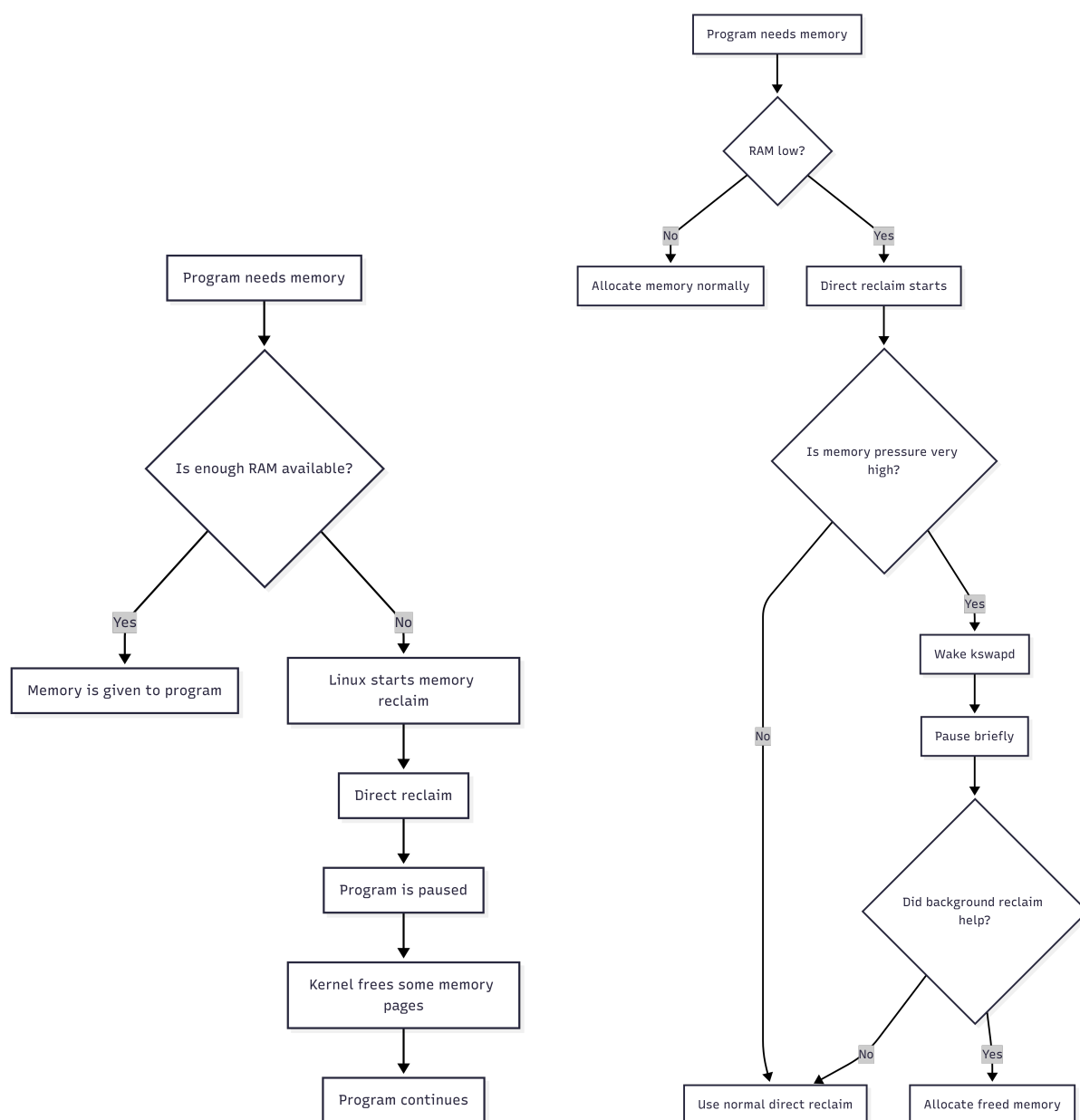
Figure 9. Left: baseline / unpatched custom build (6.8.12-baseline). Right: patched PressurePause build (6.8.12-pressurepause or 6.8.12-pressurepause+ depending on LOCALVERSION).
