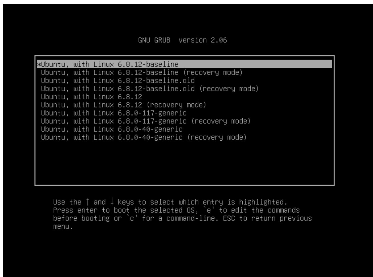
Figure 8. GRUB menu showing Ubuntu, with Linux 6.8.12-baseline selected, with recovery and fallback Ubuntu kernel entries still available.
