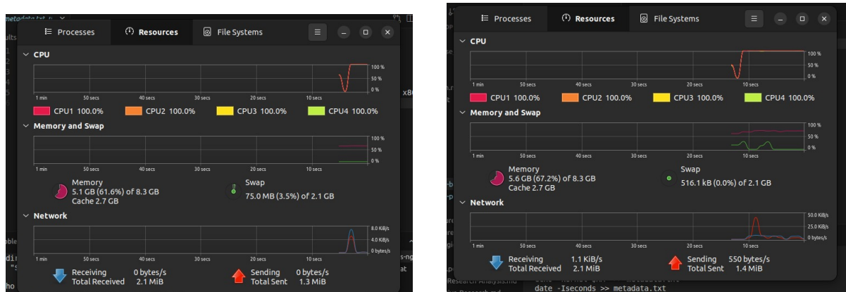
Figure 12. Left: representative benchmark / monitoring session on the baseline kernel during a stress-ng memory workload. Right: comparable session on the PressurePause kernel (same host class of workload; 120 s timeouts and tool output as in ./bench-run.sh ).
