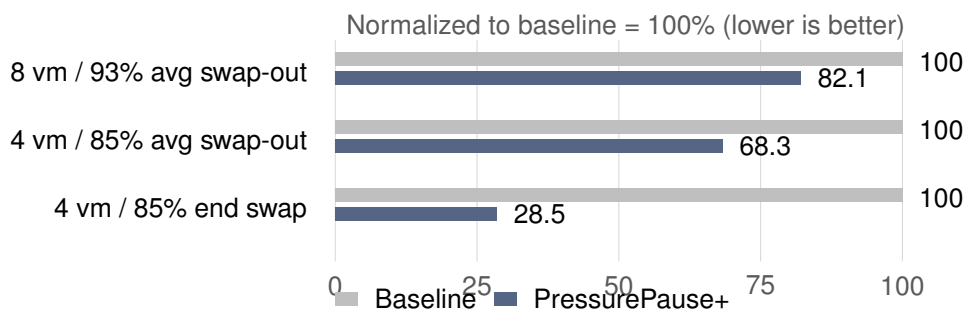
Figure 13. Visual comparison of the strongest swap-pressure improvements. Values are normalized percentages relative to the baseline run for each metric.
