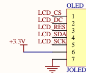
OLED
