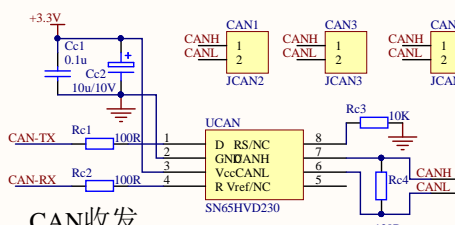
CAN收发
