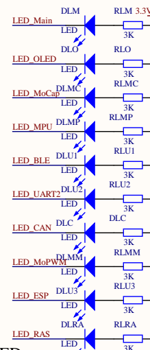
LED
