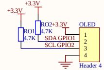
OLED
