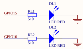
LED
