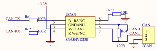
CAN收发
