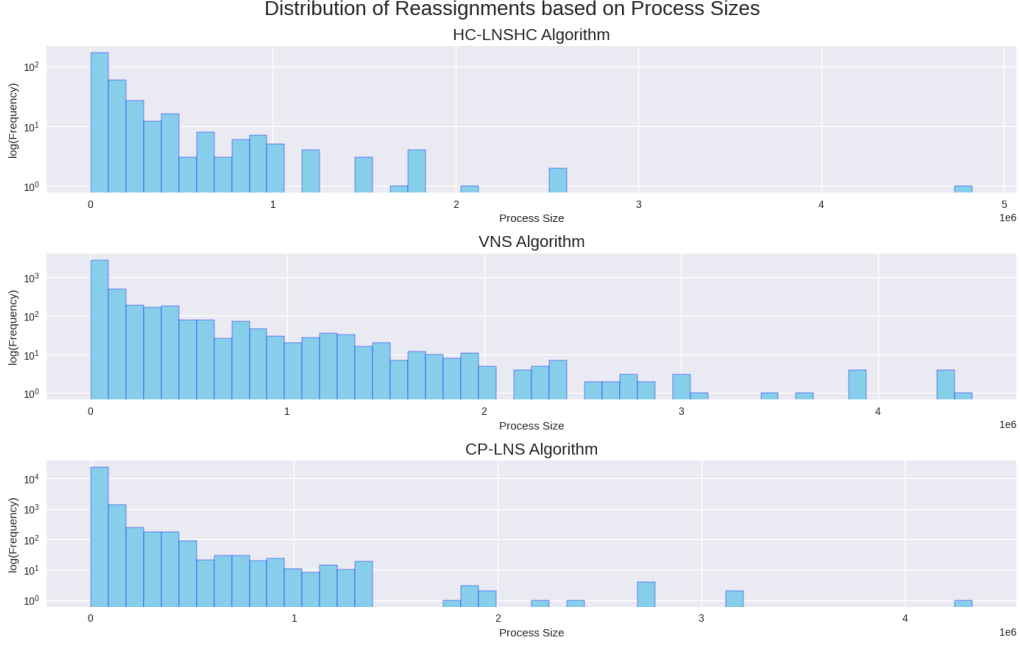
Figure 6.6: Comparison of reassignment distribution vs. Process Sizes
