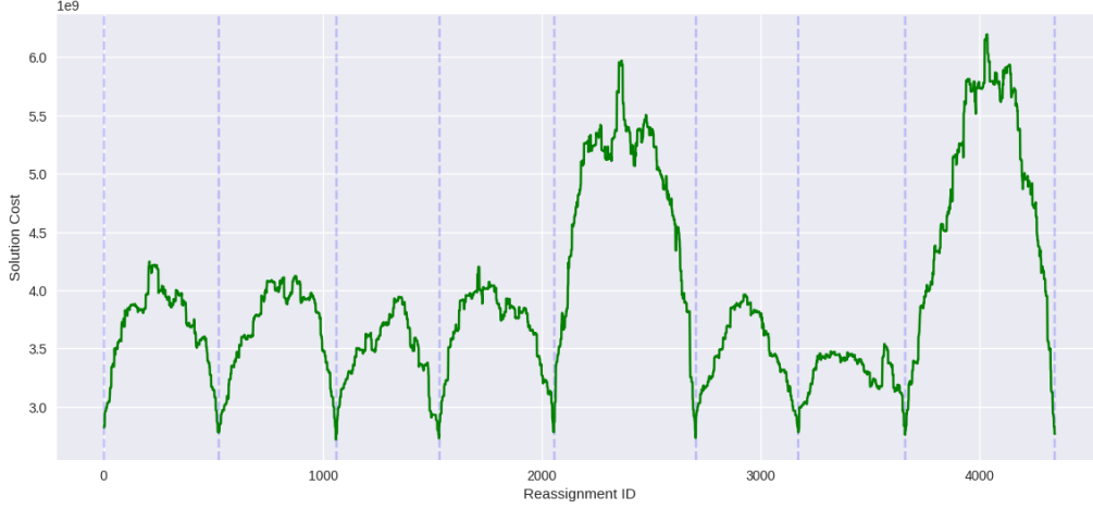
Figure 6.5: VNS Algorithm - Objective Cost over Reassignments
