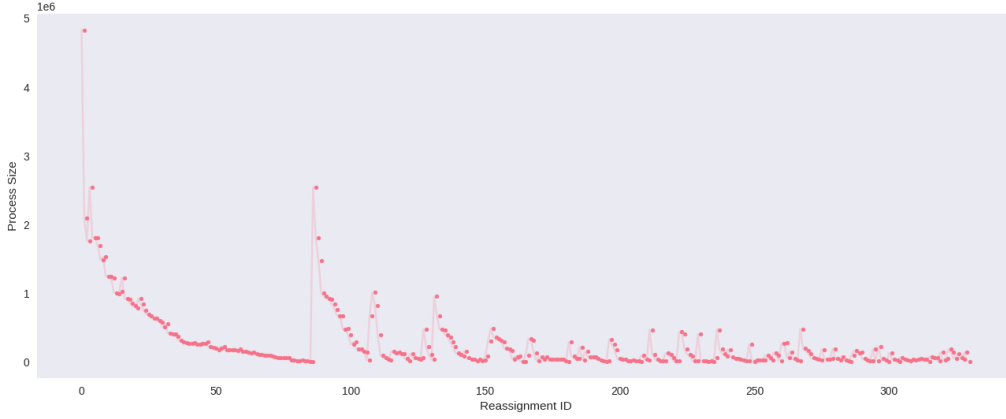
Figure 6.1: HC-LNSHC Algorithm Process Sizes of each Reassignment
