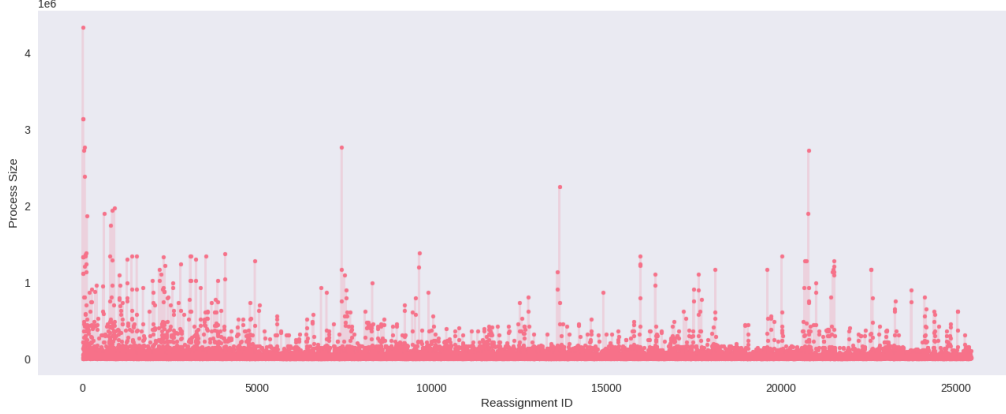
Figure 6.3: CP-LNS Algorithm Process Sizes of each Reassignment
