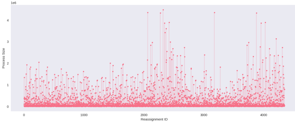
Figure 6.2: VNS Algorithm Process Sizes of each Reassignment
