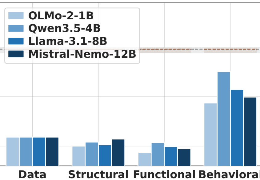
Base Model
