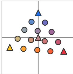
MDS 1
