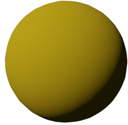
(b) Cook-Torrance
