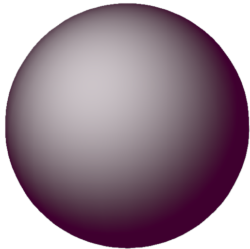
(b) Blinn-Phong
