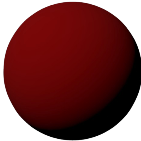
(b) Cook-Torrance
