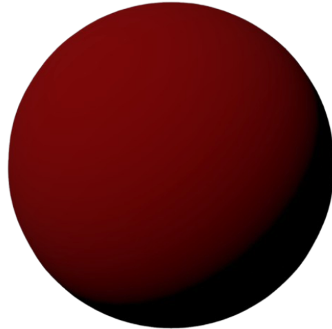
(b) Cook-Torrance
