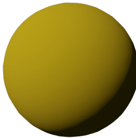
(b) Cook-Torrance
