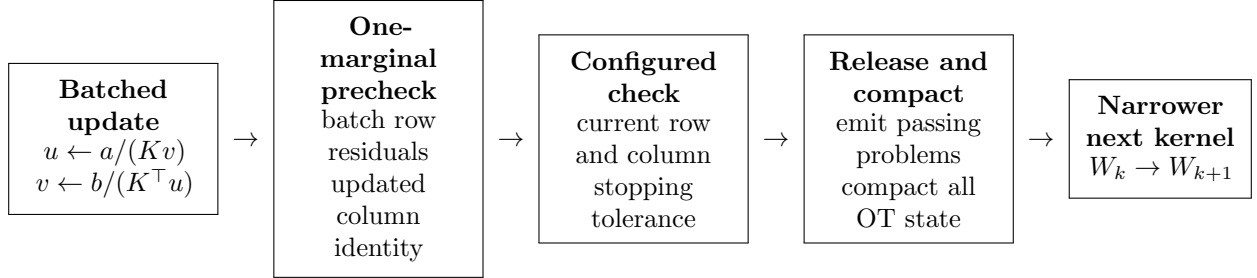
Figure 1: DrainSinkhorn’s execution loop. The preliminary check using the current marginals avoids many full plan evaluations. Problems that pass the two-marginal verifier leave every per-problem tensor; the next batched update processes only the survivors.
