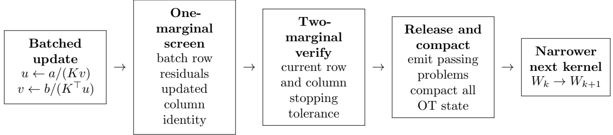
Figure 1: DrainSinkhorn’s execution loop. The one-marginal screen selects candidates for full verification but never authorizes release. A problem leaves the batch only after passing the two-marginal stopping rule, after which every associated tensor is compacted before the next update.
