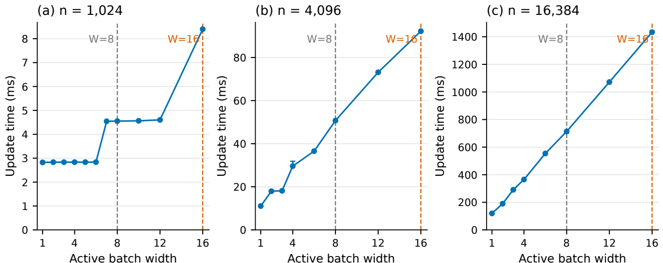
Figure 2: A100 packed-update time versus active batch width on synthetic tensors with feature dimension 500, column tile 64, and cost scale 1. Points show medians and interquartile ranges from 30 repeats, with panel-specific millisecond scales. Vertical guides locate W = 8 and W = 16 . The sweep characterizes the width response of this configuration; the application-time reconstruction in section 5.7 uses its own matched calibration.
