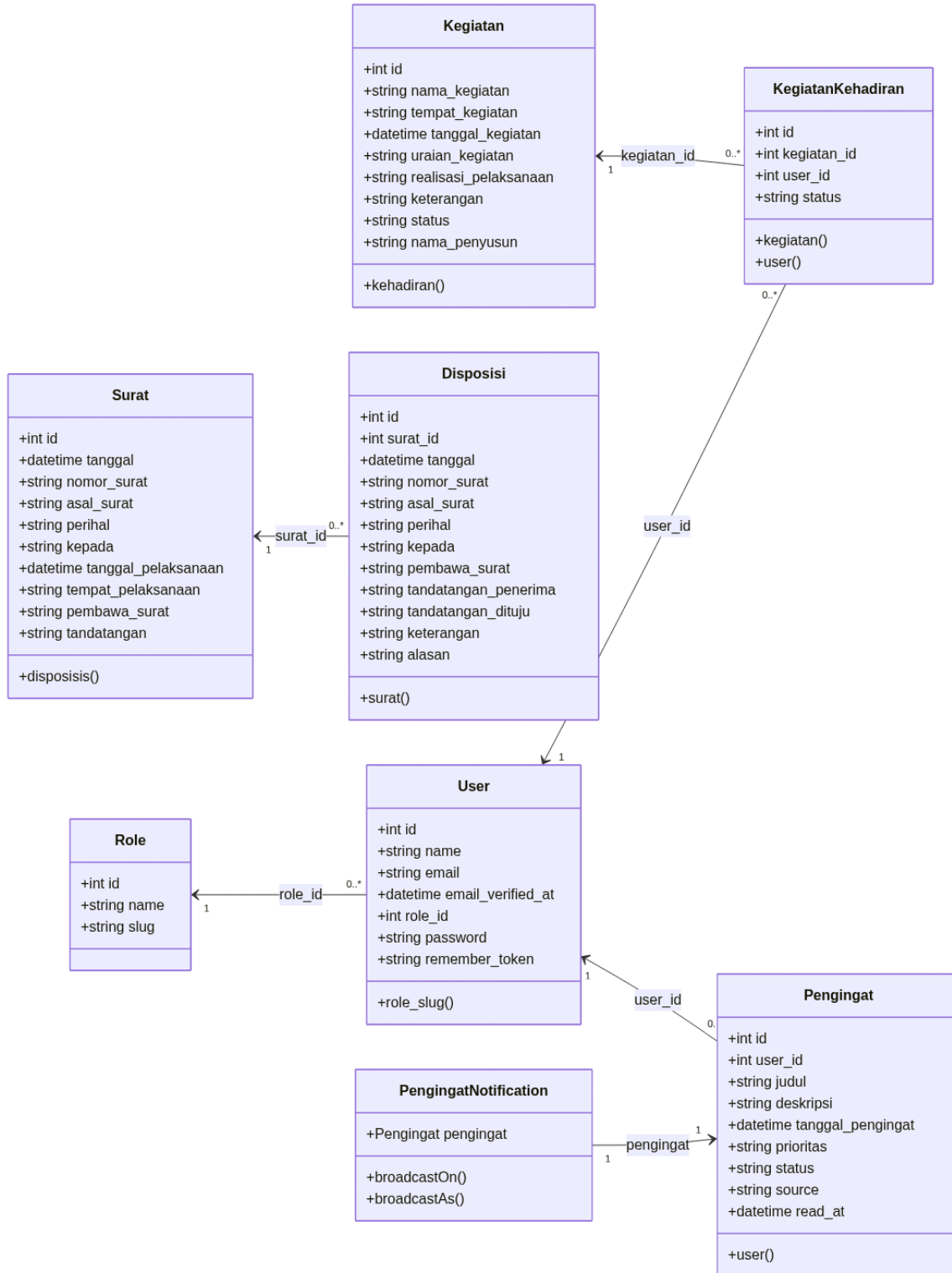
Gambar: Class Diagram
