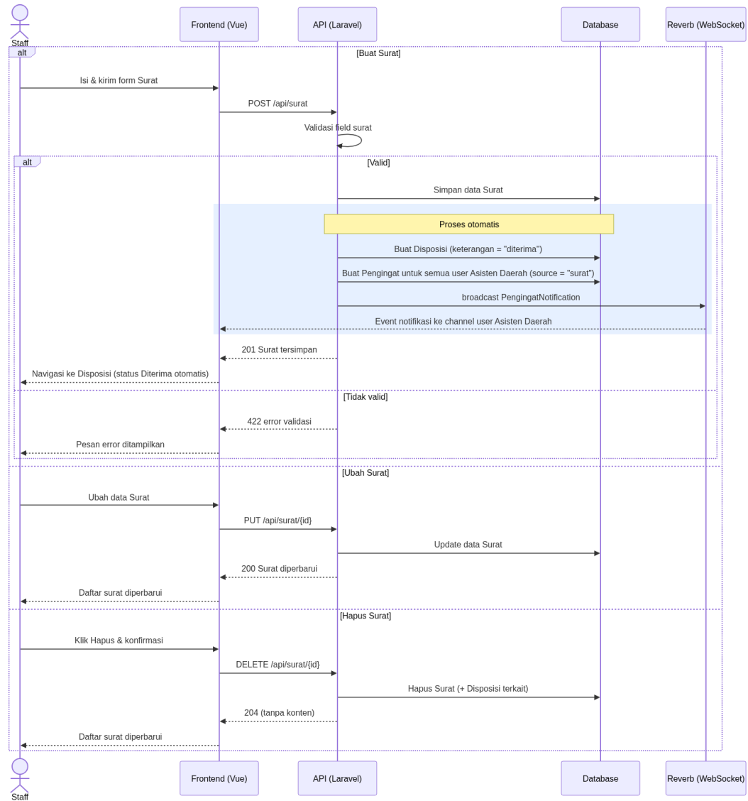
Gambar: Sequence Diagram Kelola Surat
