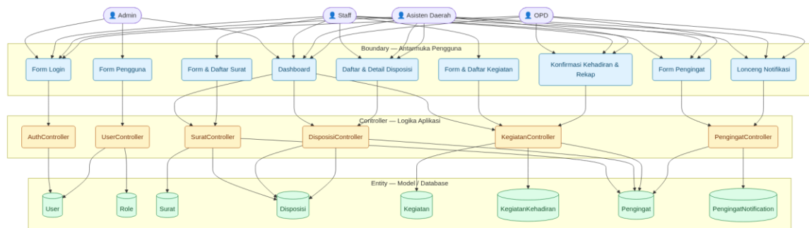
Gambar: Robustness Diagram
