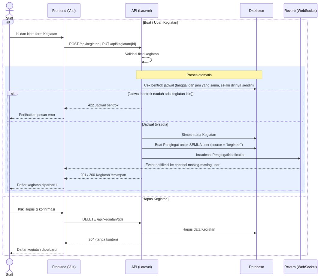
Gambar: Sequence Diagram Kelola Kegiatan
