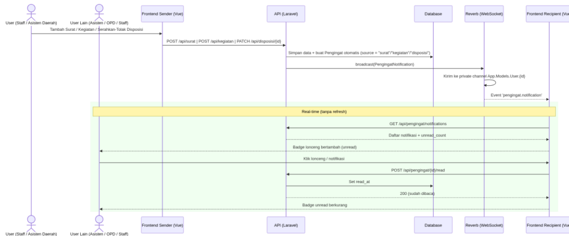
Gambar: Sequence Diagram Notifikasi Peringat Real-Time
