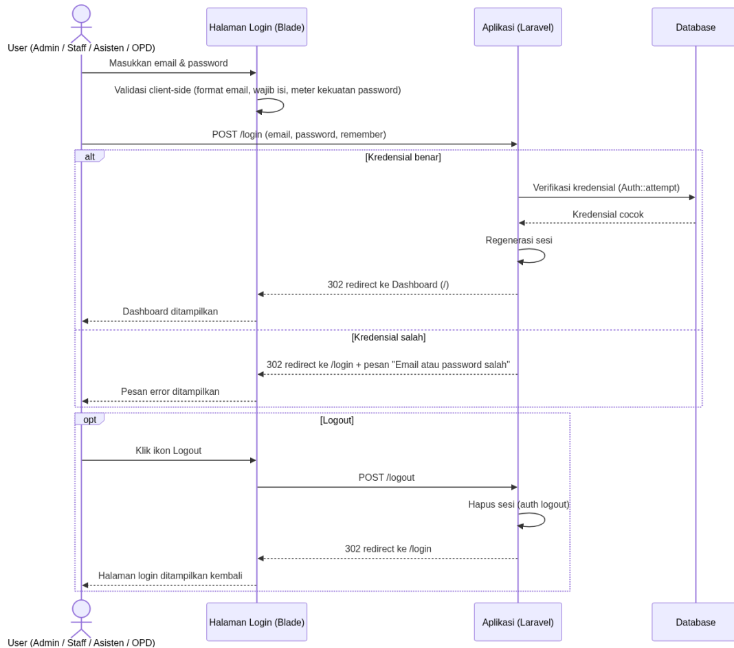
Gambar: Sequence Diagram Login & Logout
