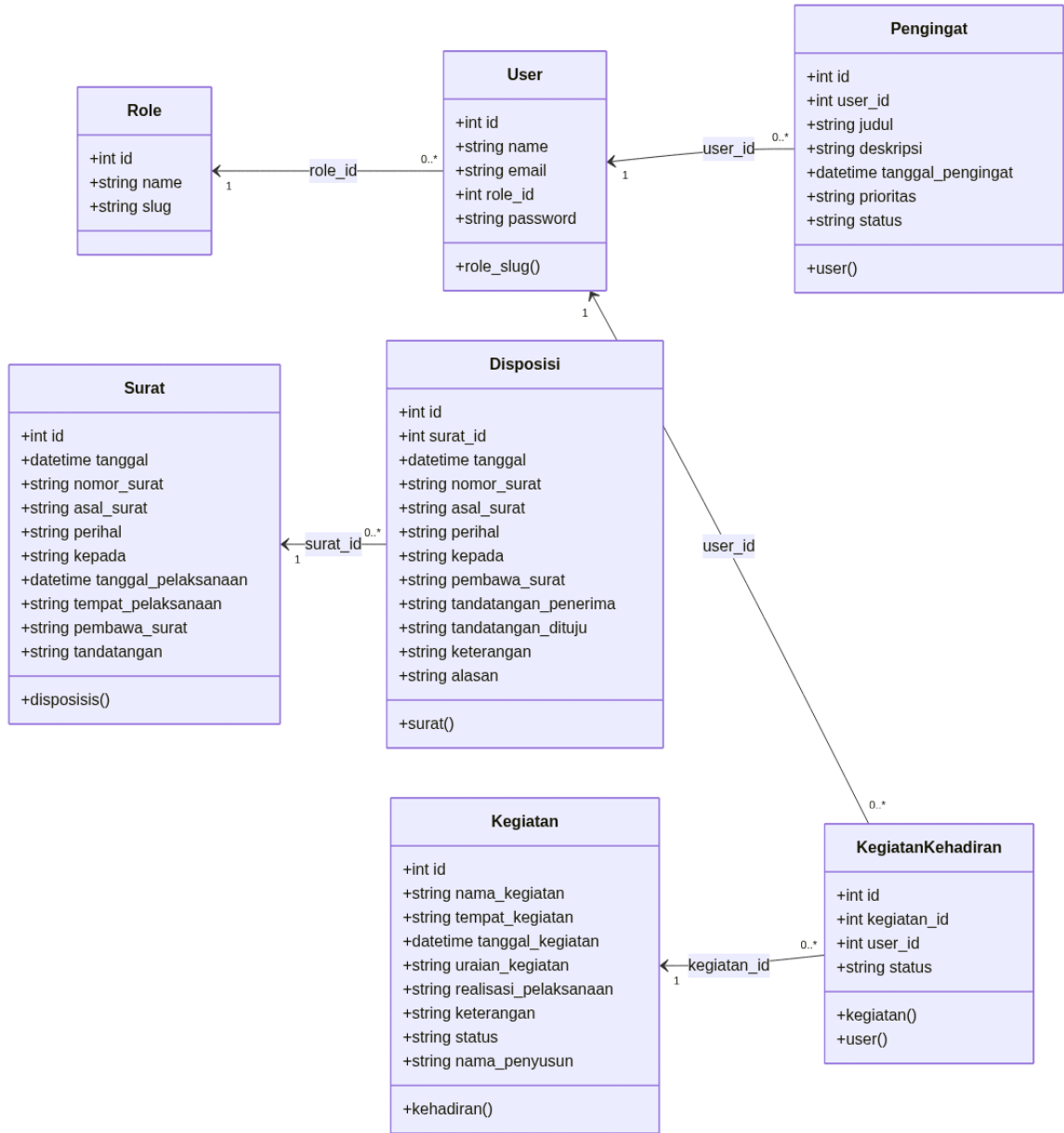
Gambar: Class Diagram
