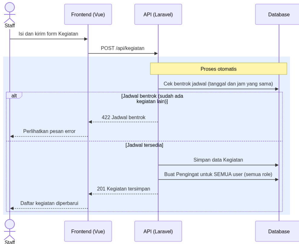
Gambar: Sequence Diagram Menambah Kegiatan
