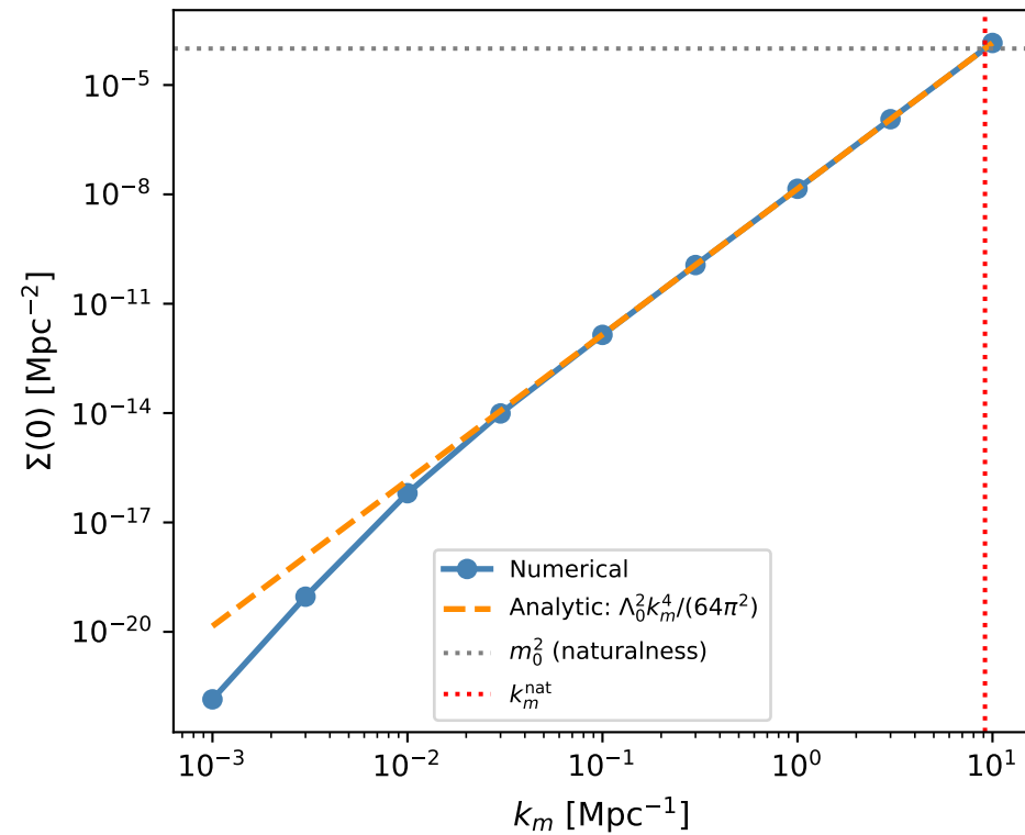
Self-energy at p = 0
