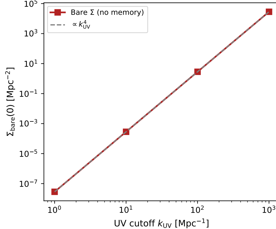
Quartic UV divergence (no memory)
