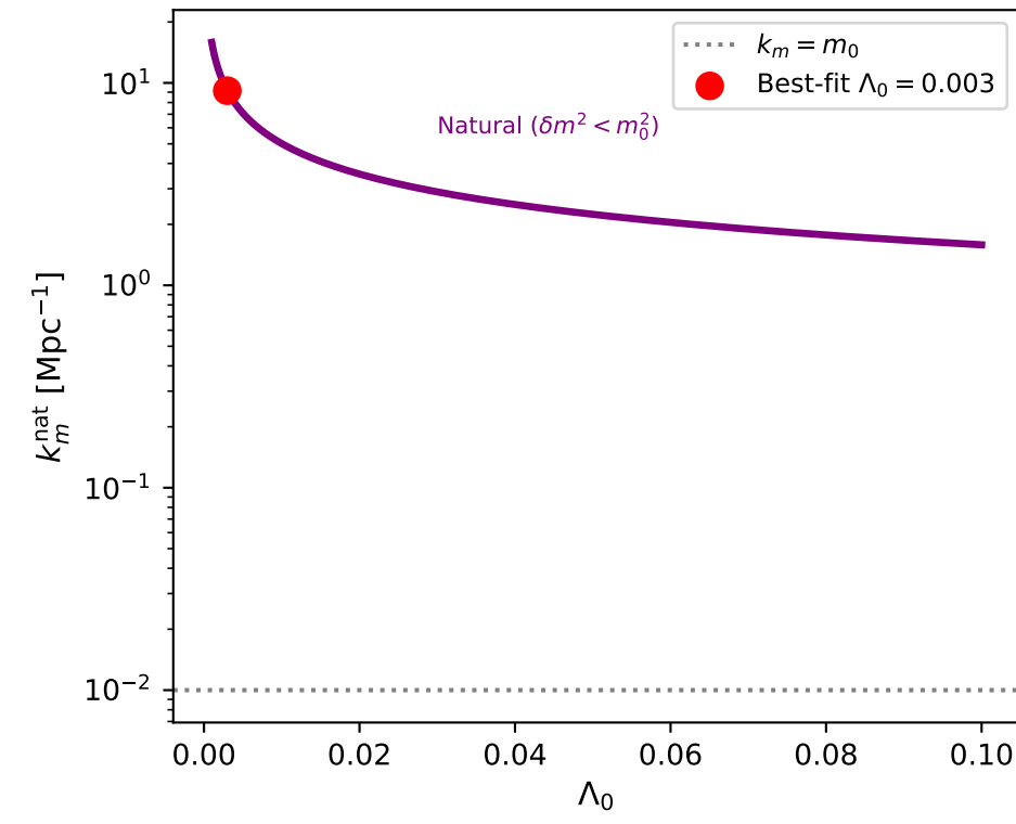
Naturalness constraint on memory scale
