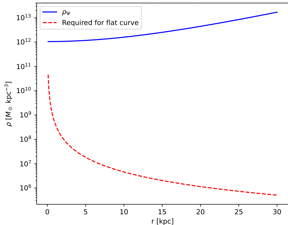
NGC6503 — \rho_\Psi vs required
