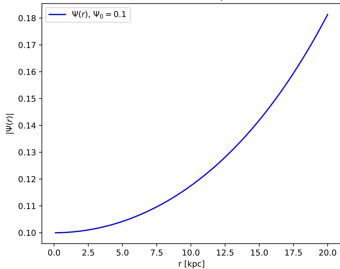
NGC6503 — Field profile
