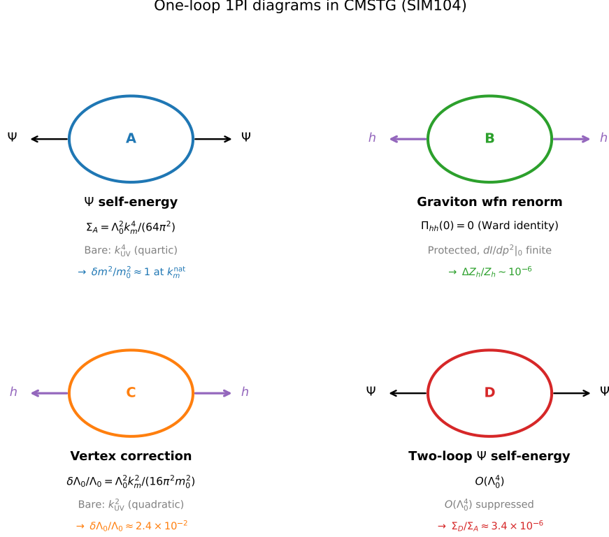
Figure 2: Diagrammatic summary of the four 1PI one-loop contributions in CMSTG (SIM104). Diagram A ( \Psi self-energy, \Lambda_0^2 k_m^4 / (64\pi^2) , regulated by memory damping), Diagram B (graviton wavefunction renormalization, \Pi_{hh}(0) = 0 by Ward identity, dI/dp^2|_0 finite), Diagram C (vertex correction \delta\Lambda_0/\Lambda_0 , slope 2), and Diagram D (two-loop \Psi self-energy, O(\Lambda_0^4) , regulated by memory). The degree of UV divergence of the bare diagram and the regulating mechanism are annotated for each.
