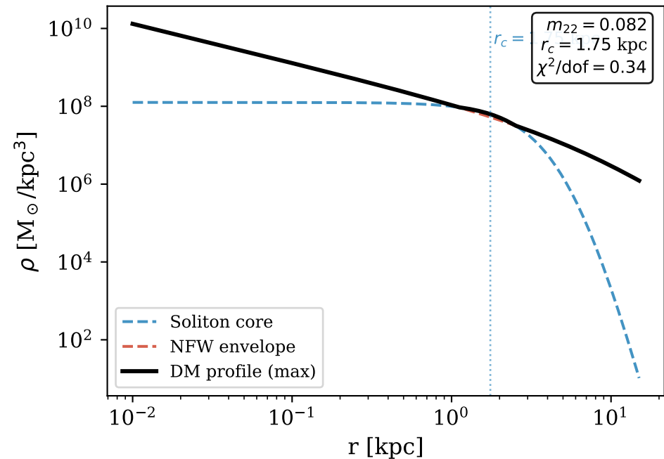
SIM118: DM Density Profile (NGC 2403 best-fit)
