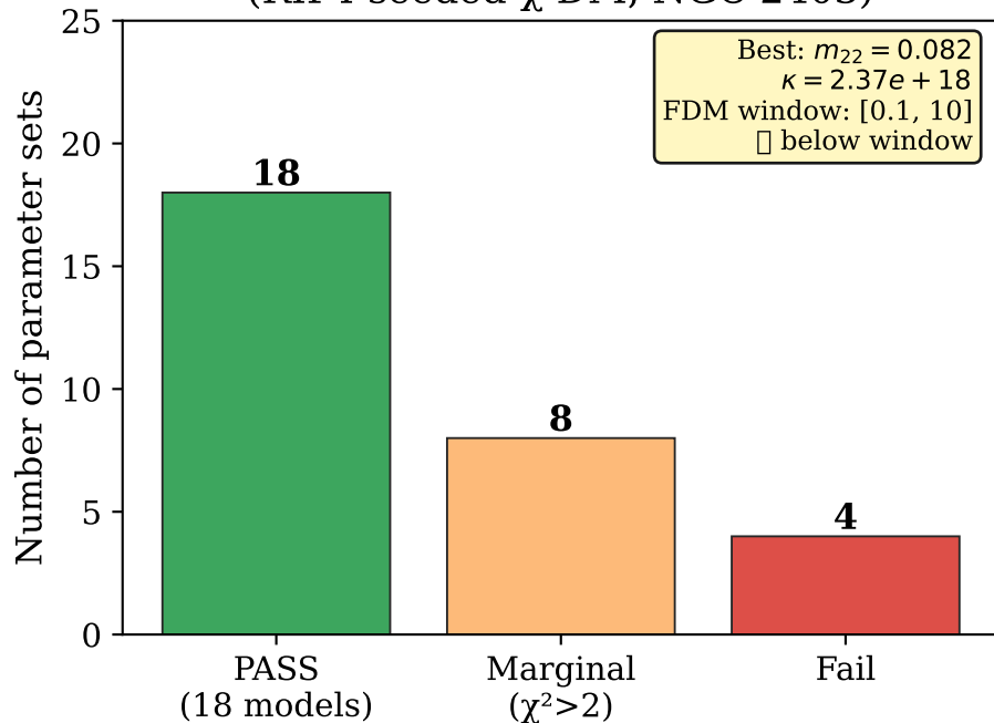
SIM118: Parameter Grid Results (RIFT-seeded \chi DM, NGC 2403)
