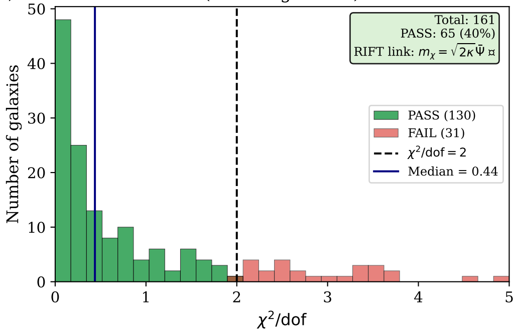
SIM119: \chi^2/\text{dof} Distribution ( N=161 galaxies)
