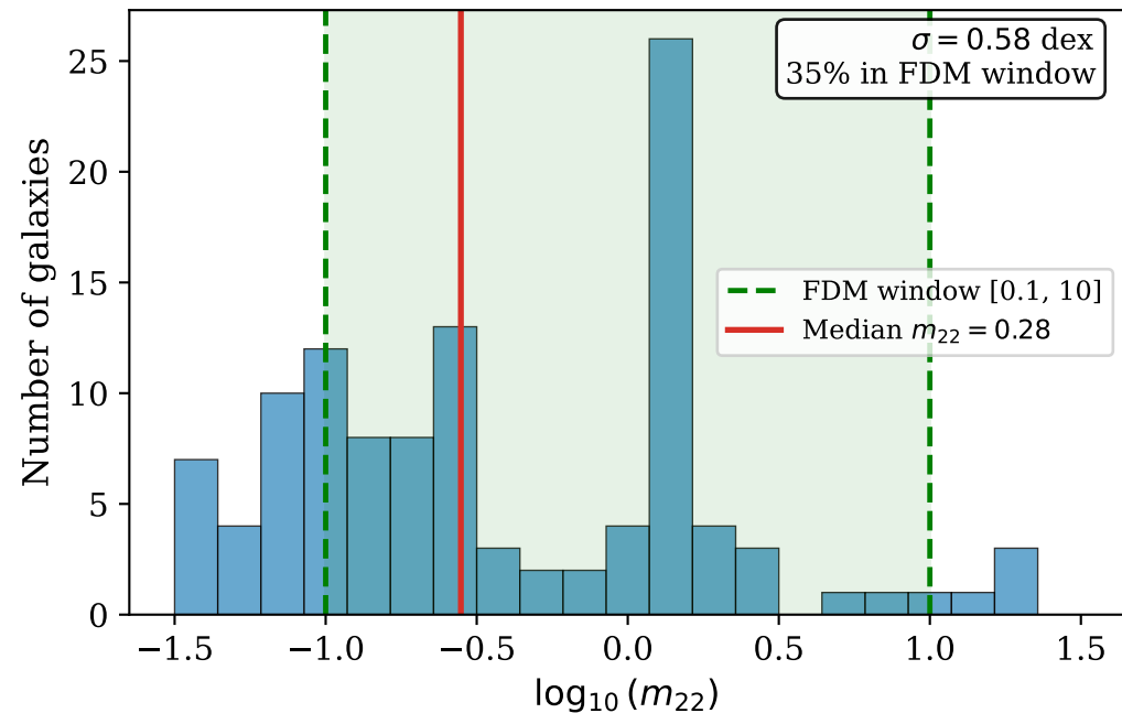
SIM119: m_{22} Distribution (SPARC, N = 161 constrained)
