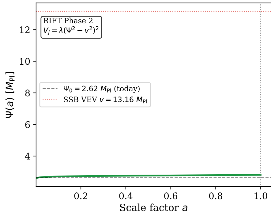
Quintessence field \Psi(a)
