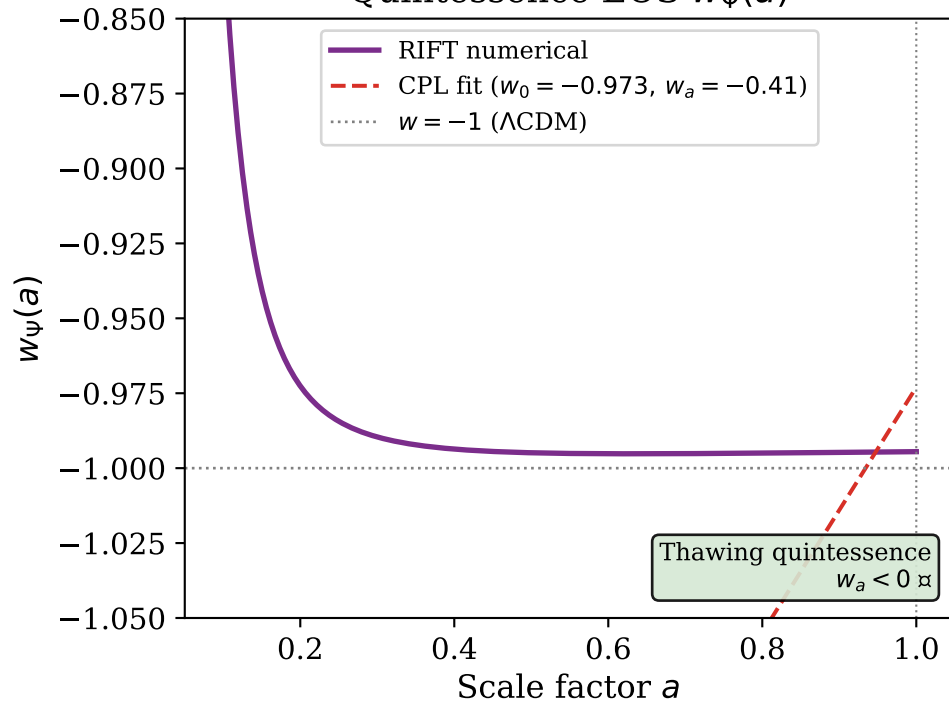
Quintessence EOS w_\Psi(a)
