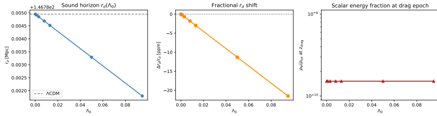
Figure 9: Sound horizon r_d as a function of \Lambda_0 (SIM101), computed with N_{\text{eff}} = 3.046 , T_{\gamma,0} = 2.7255 \text{ K} , and z_{\text{drag}} = 1059.94 . Left: r_d(\Lambda_0) with the CMSTG result (blue) and \Lambda\text{CDM} baseline (dashed). Centre: fractional shift \Delta r_d/r_d in ppm; the maximum is 21.5 ppm at \Lambda_0 = 0.095 . Right: scalar energy fraction \rho_\Psi/\rho_{\text{tot}} at the drag epoch ( \sim 10^{-10} throughout the allowed range), confirming dynamical irrelevance of \Psi at recombination. Current BAO precision is \sim 3000 \text{ ppm} .
