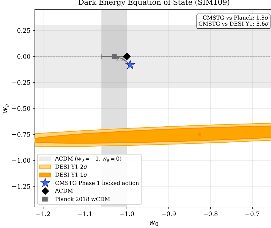
Figure 8: Dark energy equation of state (SIM109). CMSTG Phase 1 locked action (blue star) in the w_0 - w_a plane. Shaded regions: Planck 2018 wCDM 1\sigma band (grey; w_0 = -1.03 \pm 0.03 , w_a = 0 fixed), and DESI Y1 1\sigma/2\sigma contours (orange/yellow; w_0 = -0.827 \pm 0.060 , w_a = -0.75 \pm 0.29 ). CMSTG is 1.3\sigma consistent with Planck and 3.6\sigma from the DESI Y1 central value.
