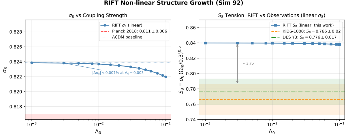
Figure 3: RIFT non-linear structure growth (Sim 92). Left : Linear \sigma_8 as a function of \Lambda_0 at the SIM90 joint best-fit cosmology ( H_0 = 67.59 , \Omega_m = 0.312 ). The RIFT curve is nearly flat; the annotation marks |\Delta\sigma_8| < 0.007\% at the BAO best-fit coupling \Lambda_0 = 0.003 . The Planck 2018 1\sigma band is shown in red. Right : Linear S_8 \equiv \sigma_8(\Omega_m/0.3)^{0.5} vs \Lambda_0 compared to KiDS-1000 [Asgari et al., 2021] and DES Y3 [Abbott et al., 2022] constraints. The pre-existing \sim 3.7\sigma gap between the RIFT/ \Lambda CDM baseline ( S_8 = 0.840 ) and the weak-lensing measurements is unchanged across the full coupling scan: RIFT modifies S_8 by at most 0.002 at \Lambda_0 = 0.1 , two orders of magnitude below the discrepancy.
