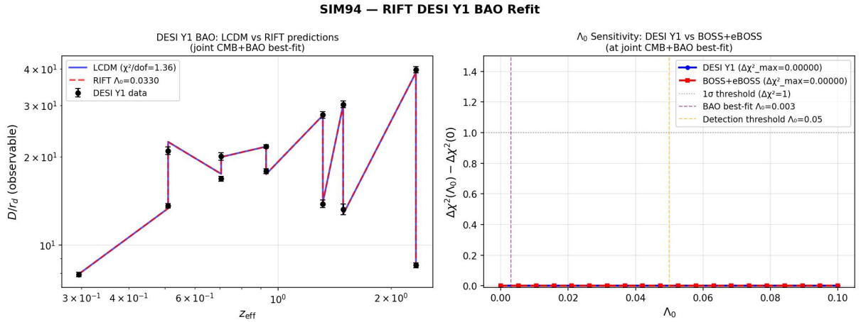
Figure 4: RIFT vs \Lambda CDM fit to DESI Y1 BAO measurements (Sim 94). 13 data points across 7 tracer bins, 0.3 \leq z \leq 2.33 . Both models give identical \chi^2/\text{dof} = 1.36/10 . The 2–3 \sigma tension at z = 0.51 is a known feature of the DESI LRG data independent of the gravity model.
