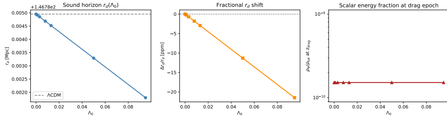
Figure 9: Sound horizon r_d as a function of \Lambda_0 (SIM101), computed with N_{\text{eff}} = 3.046 , T_{\gamma,0} = 2.7255 \text{ K} , and z_{\text{drag}} = 1059.94 . Left: r_d(\Lambda_0) with the CMSTG result (blue) and \Lambda CDM baseline (dashed). Centre: fractional shift \Delta r_d / r_d in ppm; the maximum is 21.5 ppm at \Lambda_0 = 0.095 . Right: scalar energy fraction \rho_\Psi / \rho_{\text{tot}} at the drag epoch ( \sim 10^{-10} throughout the allowed range), confirming dynamical irrelevance of \Psi at recombination. Current BAO precision is \sim 3000 \text{ ppm} .
