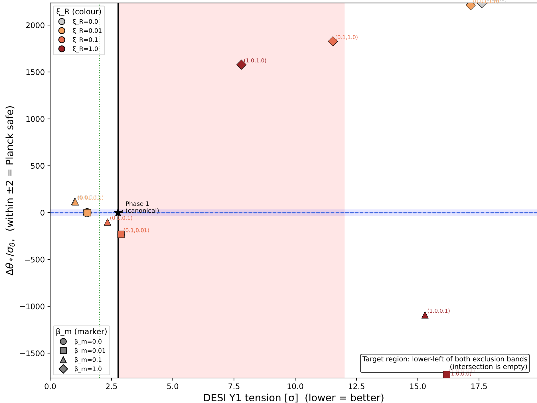
SIM144: DESI tension vs CMB acoustic angle All 16 cases; Phase 1 reference and theorem exclusion regions shown
