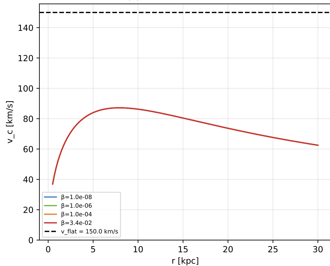
(c) Rotation curves vs r
