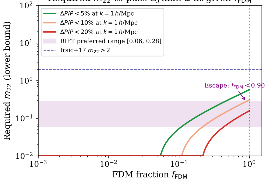
Required m_{22} to pass Lyman- \alpha at given f_{\text{FDM}}
