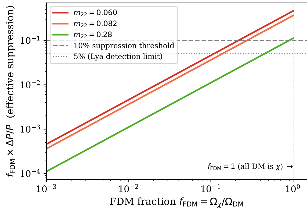
Effective Suppression vs f_{\text{FDM}} at k = 1 \text{ h/Mpc}
