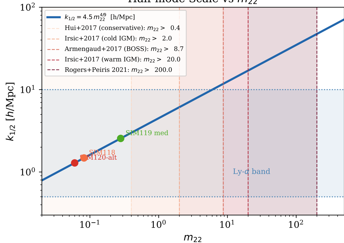
Half-mode Scale vs m_{22}
