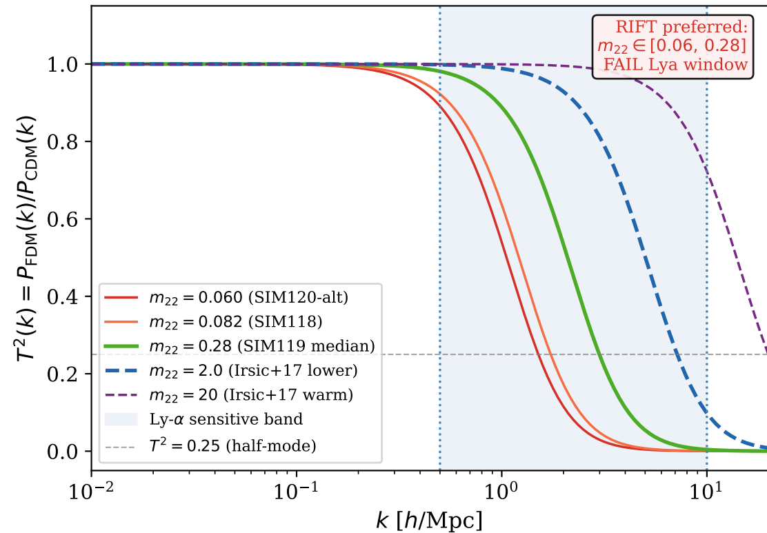
FDM Transfer Function T^2(k)
