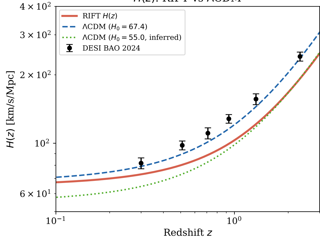
H(z) : RIFT vs \Lambda CDM
