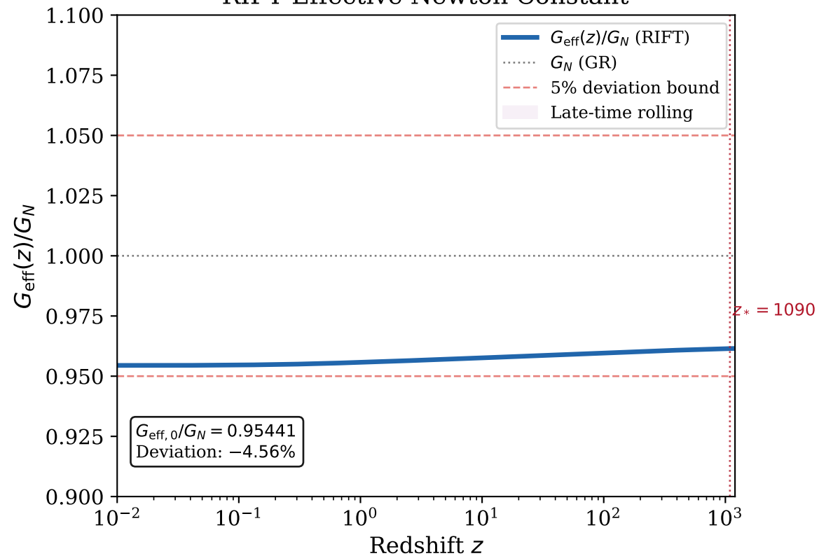
RIFT Effective Newton Constant
