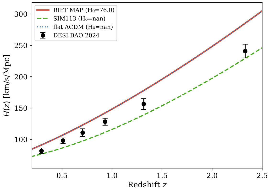
H(z) : RIFT MAP vs Data
