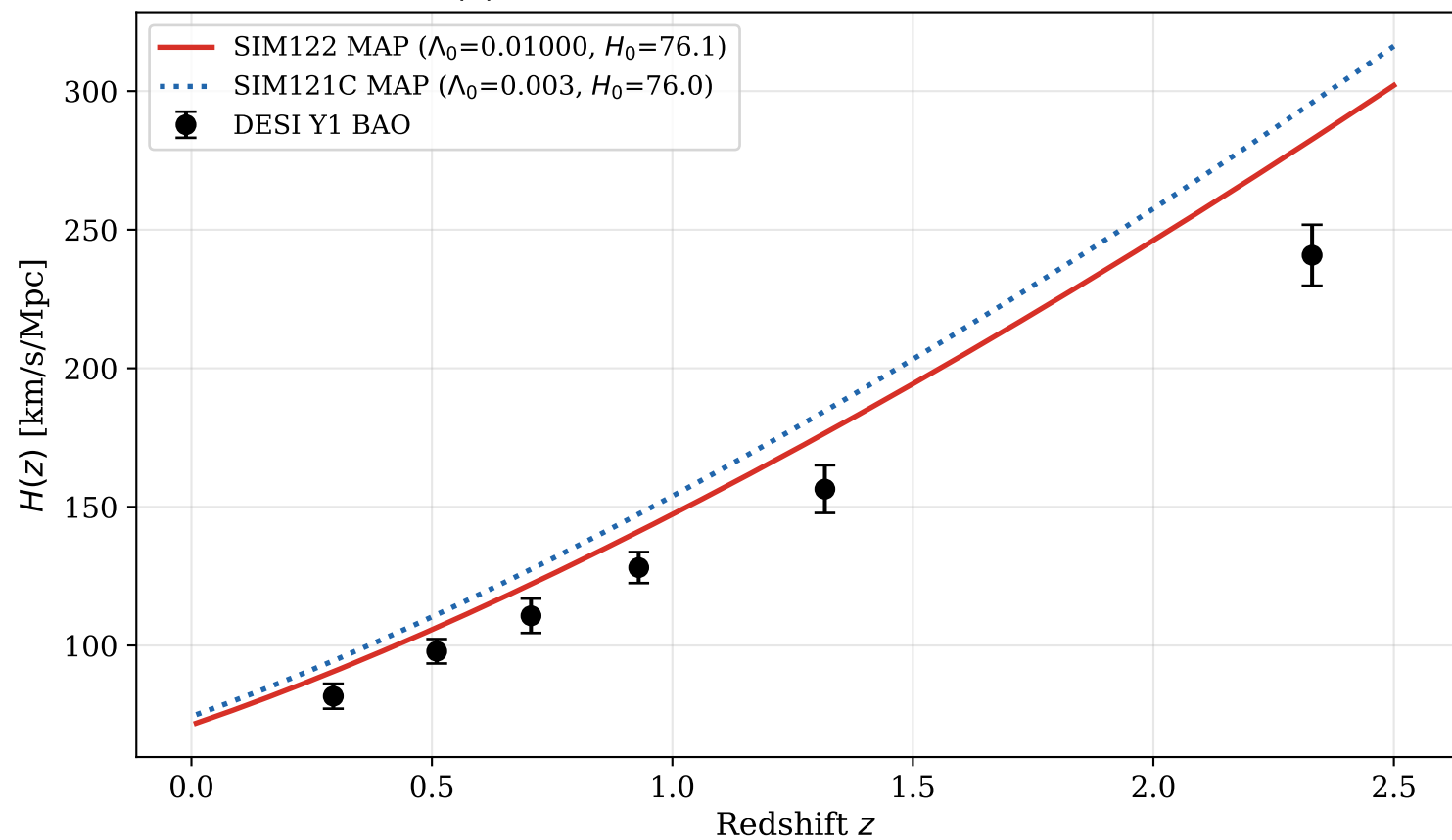
H(z) at SIM122 MAP vs SIM121C vs DESI
