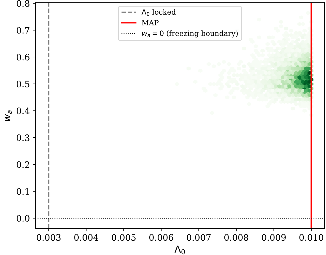
Posterior: \Lambda_0 vs w_a
