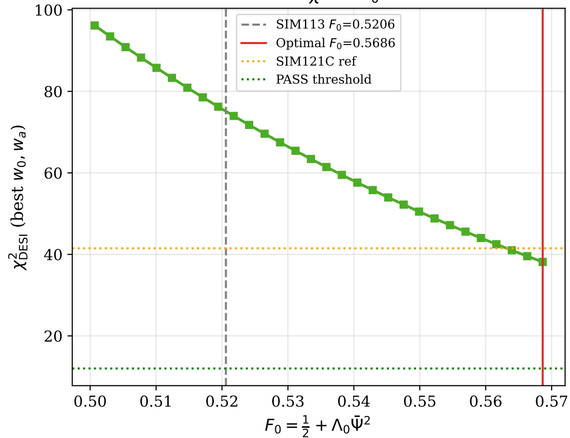
DESI \chi^2 vs F_0
