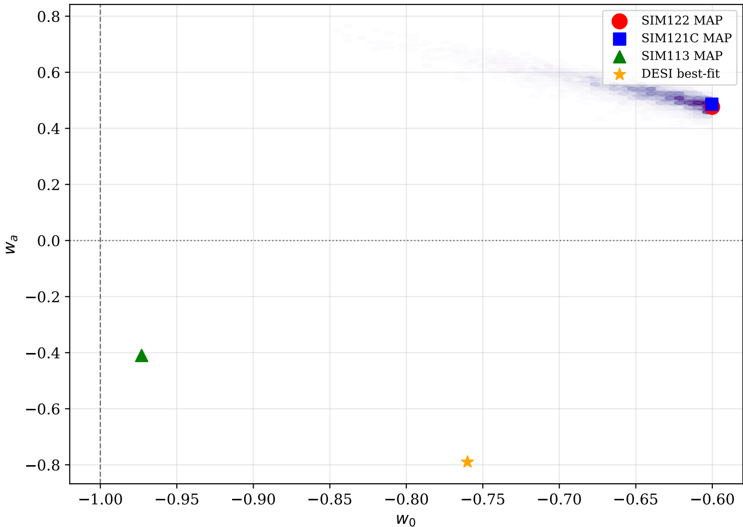
w_0 -- w_a posterior: SIM122 vs references
